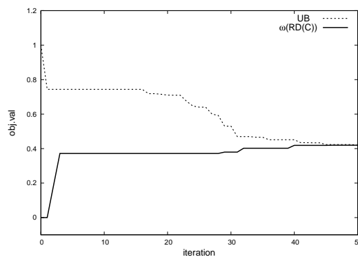
Figure 1: Behavior of SCP for Karate
